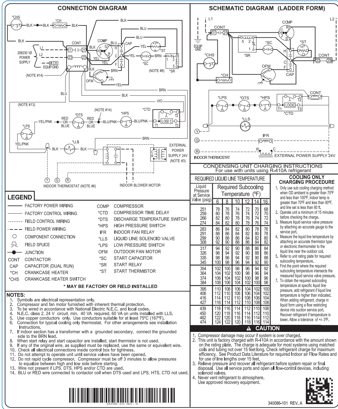
Fig. 1 – Wiring Diagram — 208/230-1 Models PA13NA, PA14NC, PA15NC, Sizes 018-060, PA16N*, Sizes 018-048, PA16N*0600
