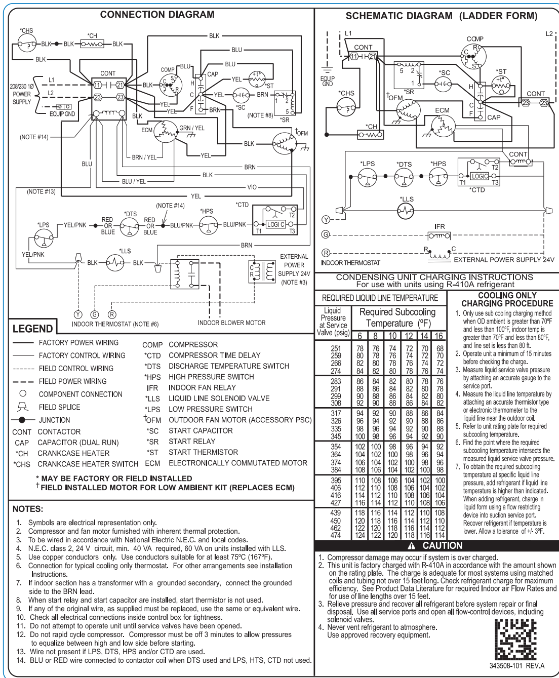
Fig. 2 – Wiring Diagram — 208/230-1 Models PA16N*060B
