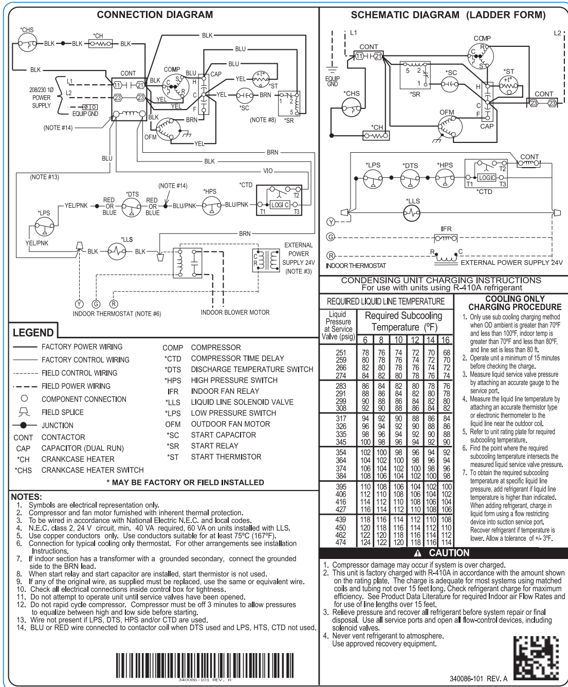
Fig. 1 – Wiring Diagram — Models PA13NA, PA14NC, PA15NC 018-060, PA16NA, Sizes 024-060 PA16NW, Sizes 018-060, 208/230-1
