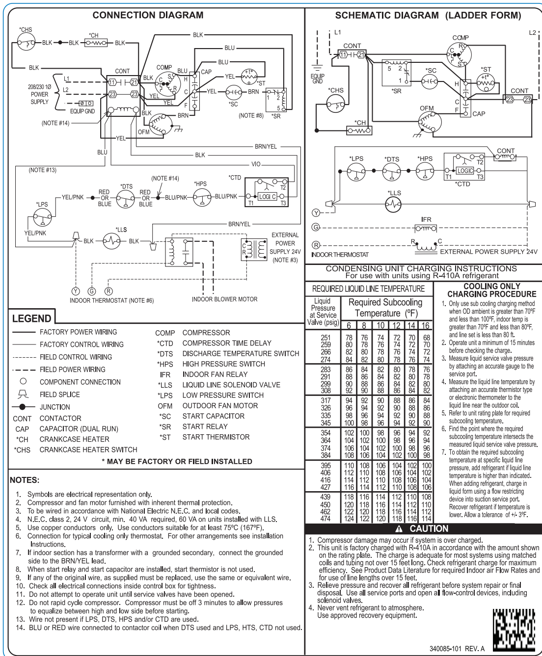
Fig. 2 – Wiring Diagram — Models PA16NA036-061, PA16NW036-060, 208/230-1 - Legacy models, no longer in production
