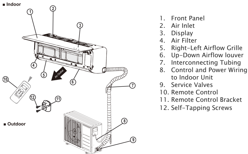
Fig. 1 — Indoor/Outdoor Unit
