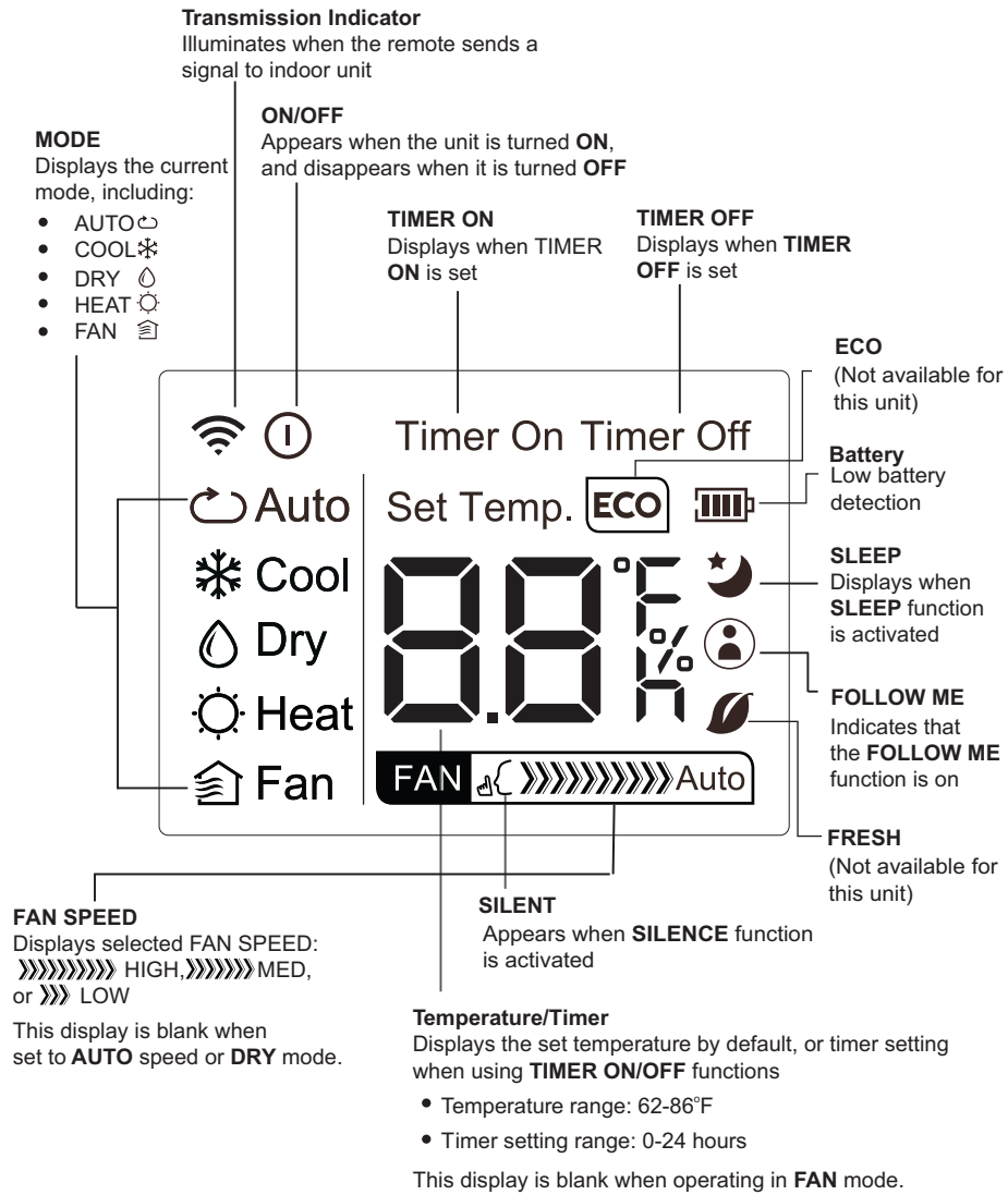
Fig. 4 — Wireless Remote Display
