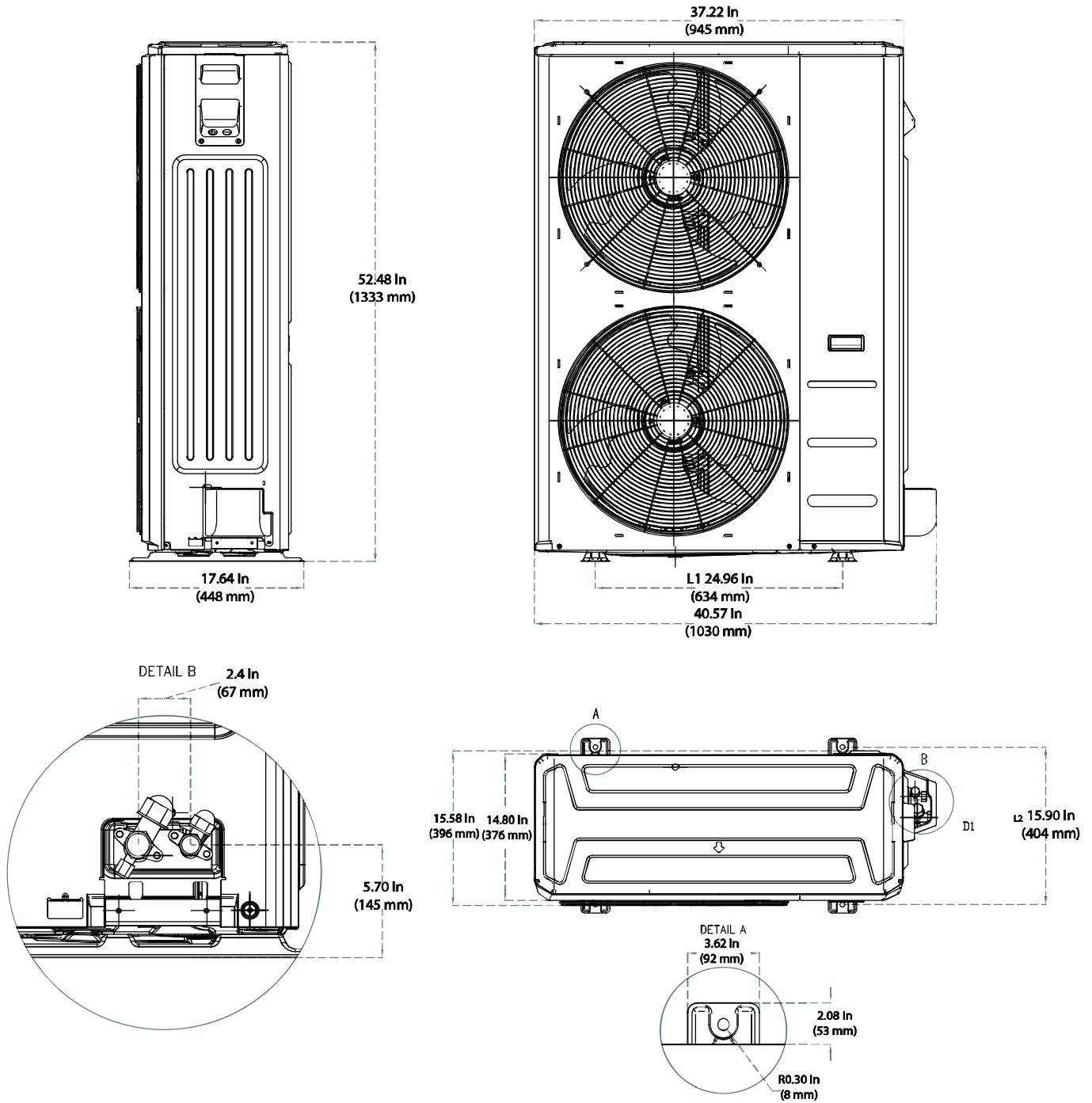
Fig. 2 – Sizes 48K–58K
